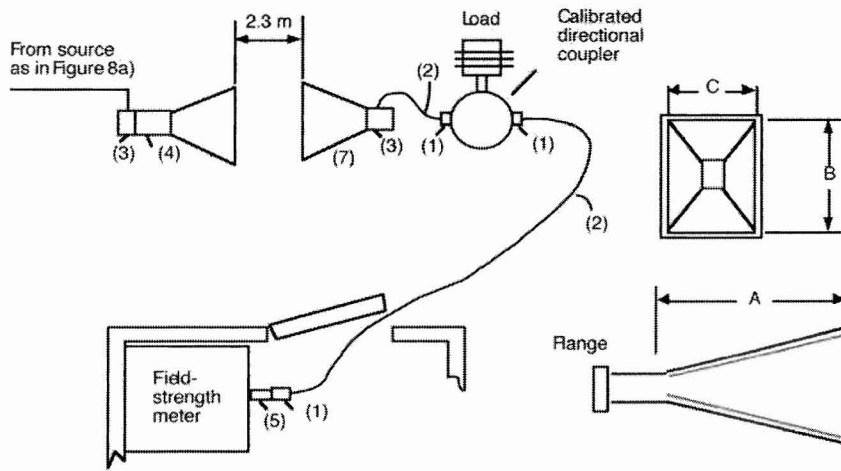
b) Enclosure free-field simulation
