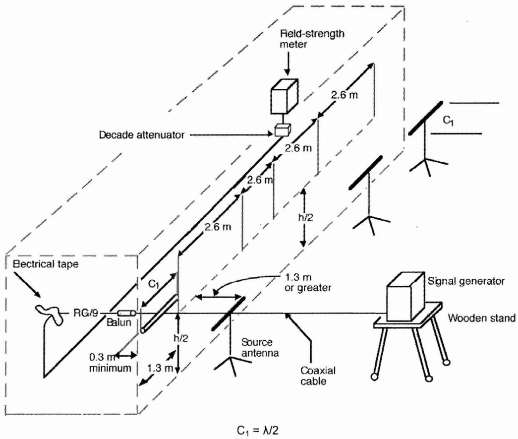
Figure 7—Measurement setup for frequencies \leq 1000 MHz
