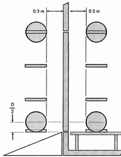
b) Door measurements
