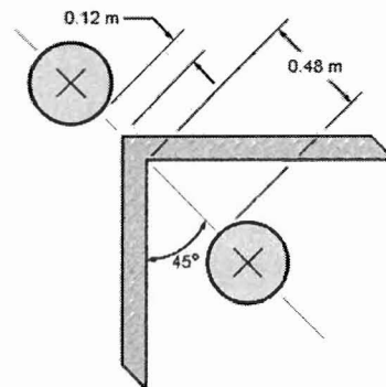
f) Fully accessible corner seam measurements
