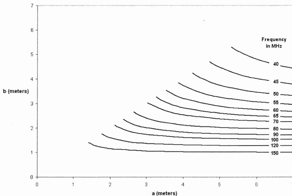
Figure 5—Lowest natural resonant frequency chart
