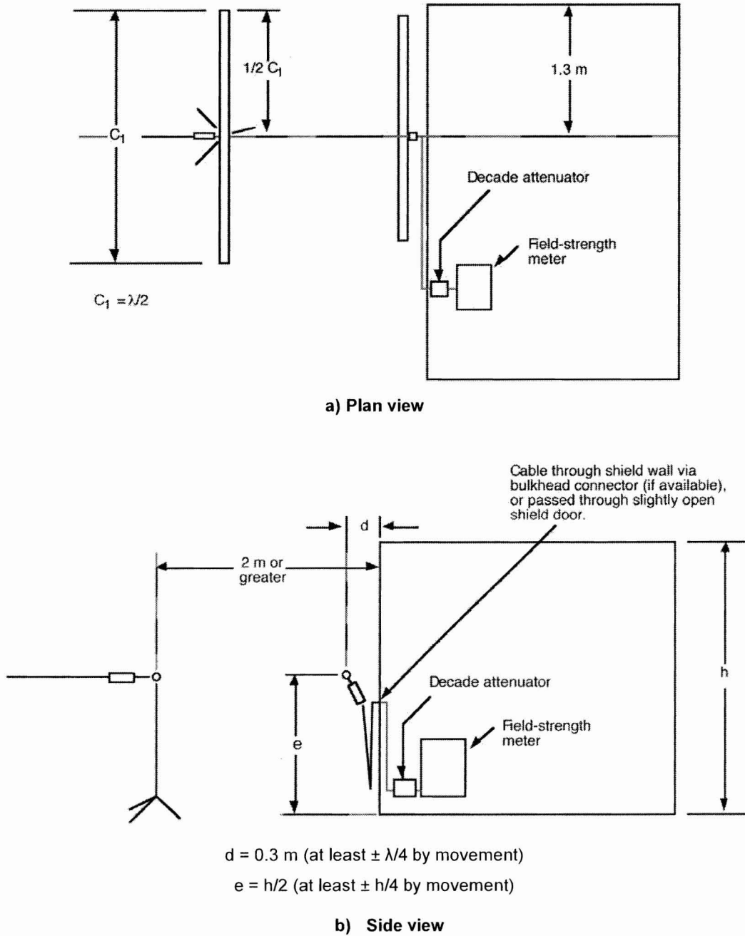
Figure 6—Reference setup for frequencies \leq 1000 MHz
