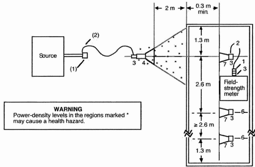
a) Broad-area microwave penetration
