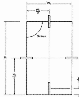
d) Panel seam measurements
