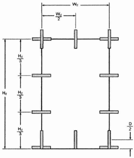
a) Single-panel entry door measurements
