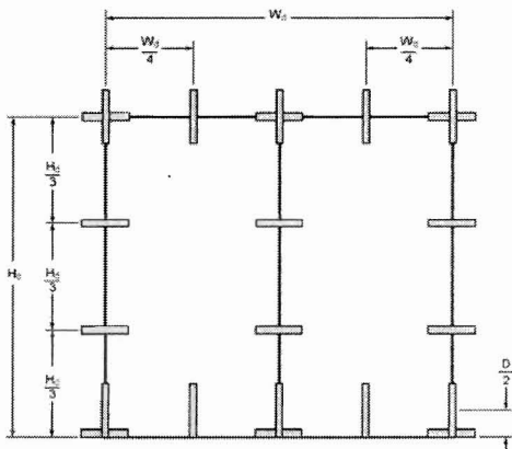
c) Double-panel entry door measurements
